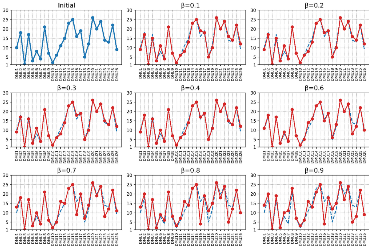
Fig. 7. Effect of variations in \beta values on final ranking (FY 2024-25)
