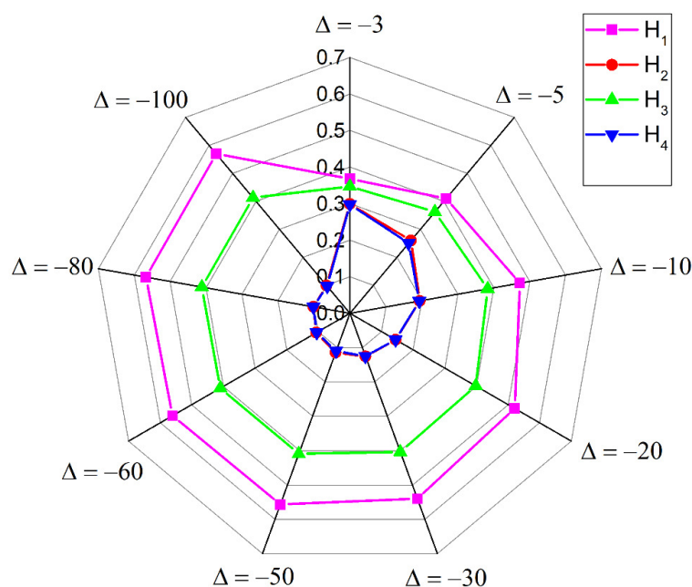
Fig. 4. Influence of \Delta under the SFRSSWA operator
