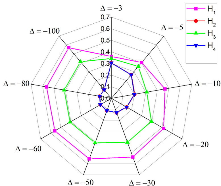
Fig. 5. Influence of \Delta under the SFRSSWG operator
