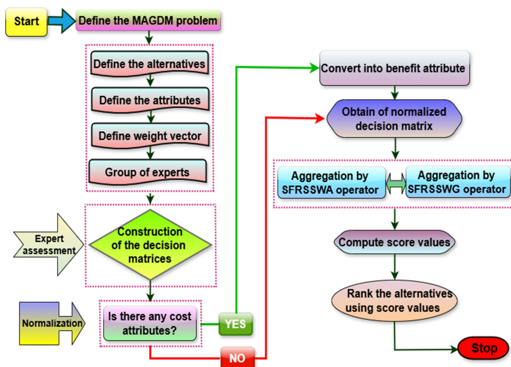
Fig. 2. Flowchart of the proposed MAGDM scheme
