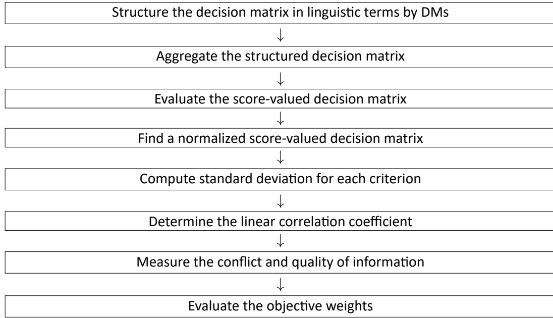
Fig. 2. Constructional framework of the CRITIC methodology
