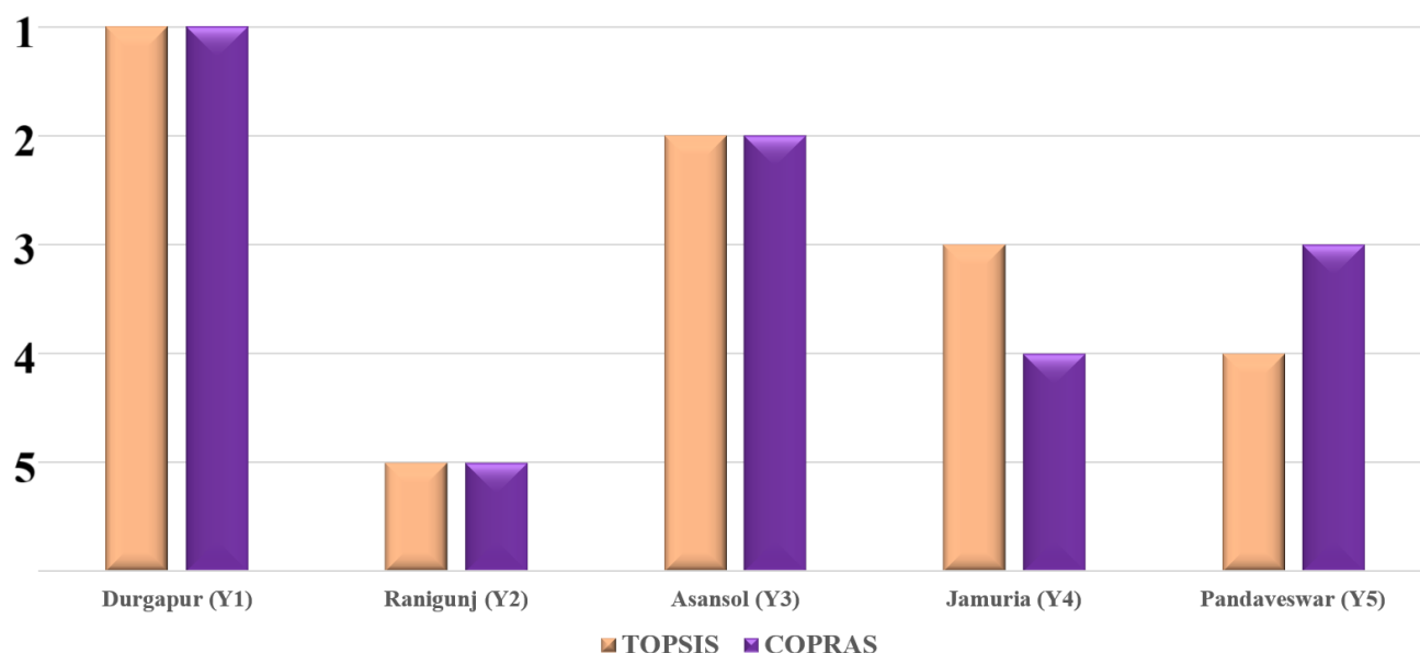
Fig. 10. Comparative analysis by TOPSIS procedure with our proposed methodology
