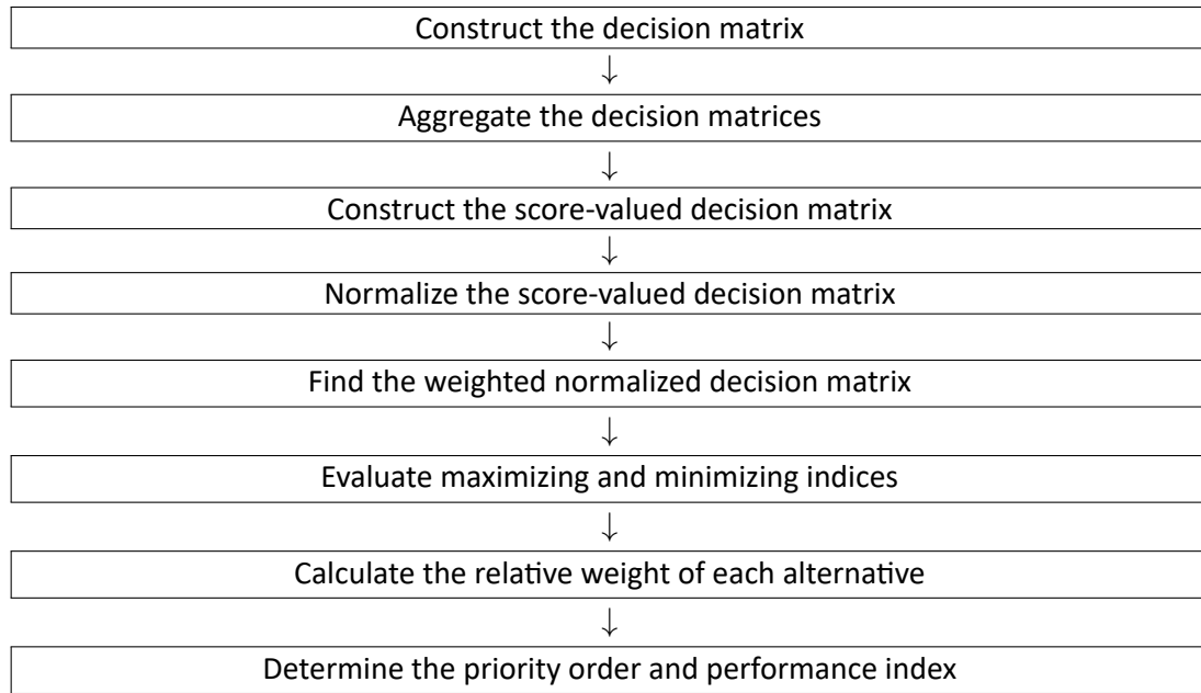
Fig. 3. Structure process of the COPRAS methodology
