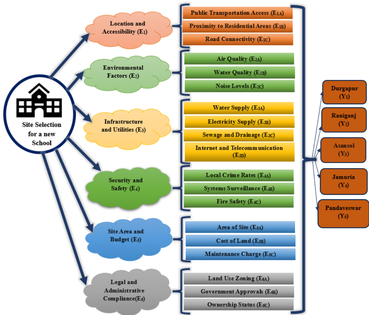
Fig. 5. Structural flowchart of the suggested model
