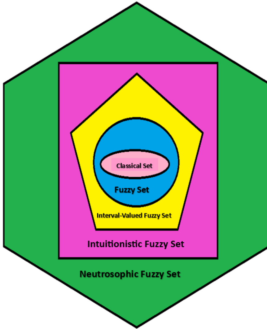
Fig. 1. Diagram of evaluation of fuzzy Sets
