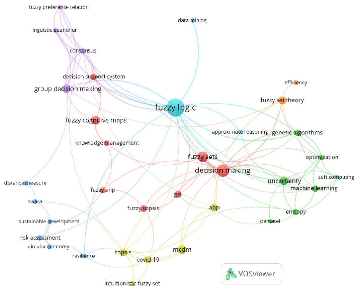
Fig. 3. Co-occurrence of author keywords of fuzzy research (minimum 5 occurrences & 100 links)
