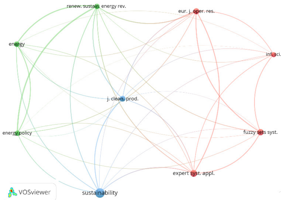
Fig. 4. Co-citation of journals of fuzzy research in Italy (minimum 100 citations & 100 links)
