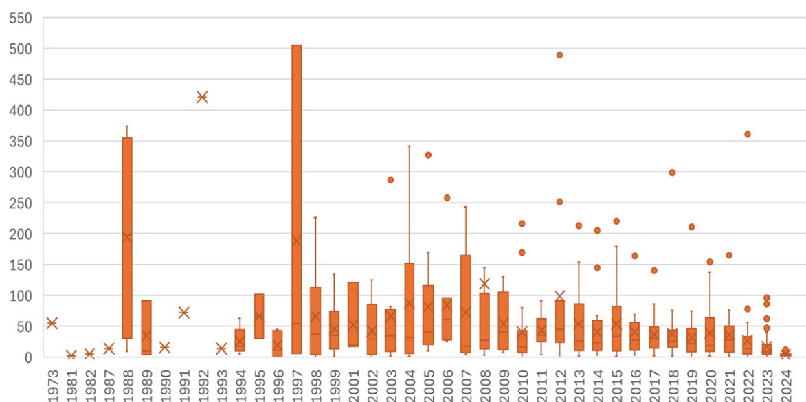
Fig. 2. Annual publication vs citation chart
